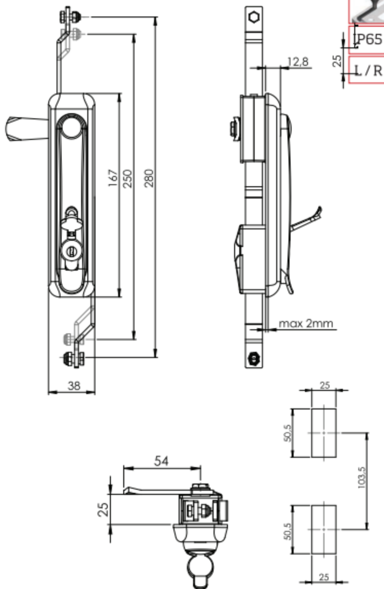
ASMA HAMILİ KİLİT PADLOCK DEVICE
