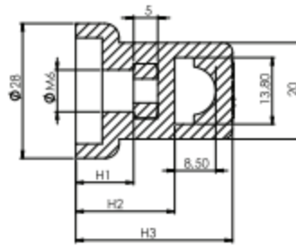
KESİT B-B CROSS SECTION B-B
