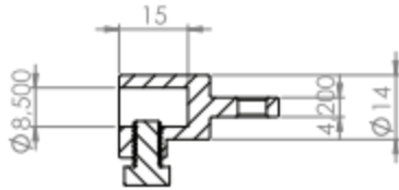
CROSS SECTION B-B
